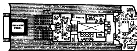
PROMENADE DECK
