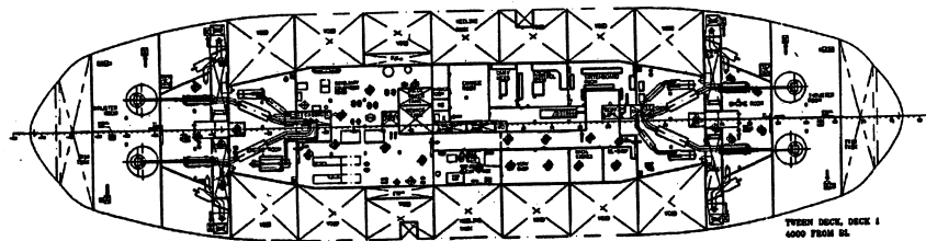
TWEEN DECK, DECK 1 4000 mm FROM SL
