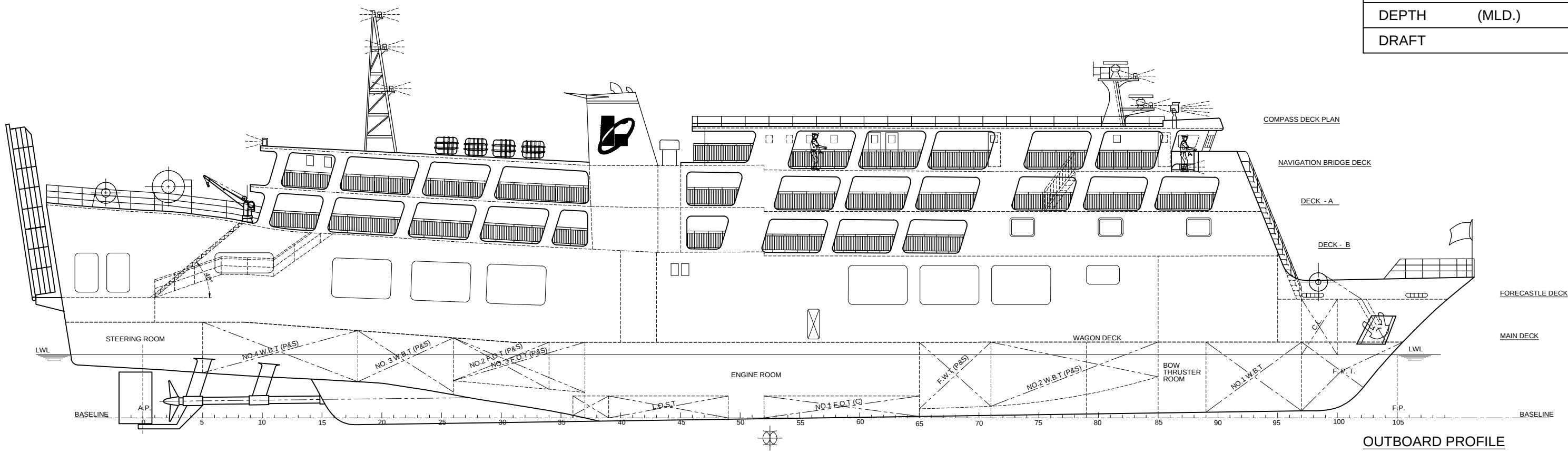
OUTBOARD PROFILE
