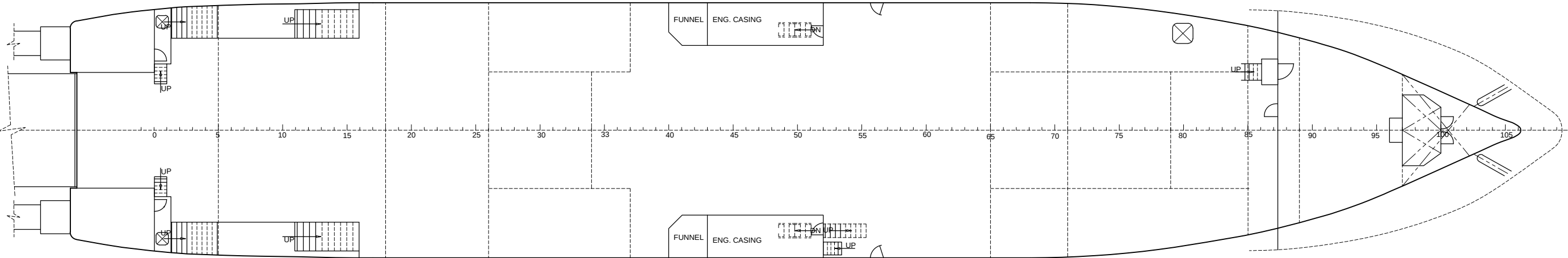
WAGON DECK PLAN
