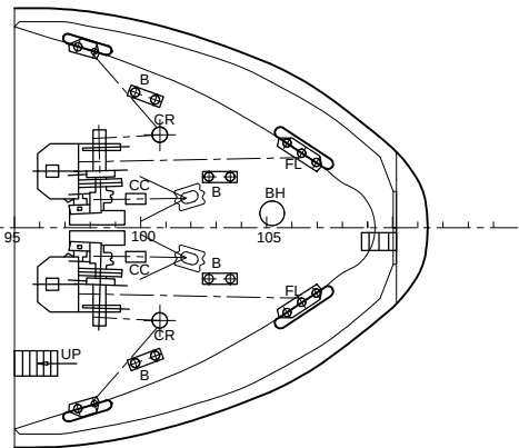
FORECASTLE DECK
