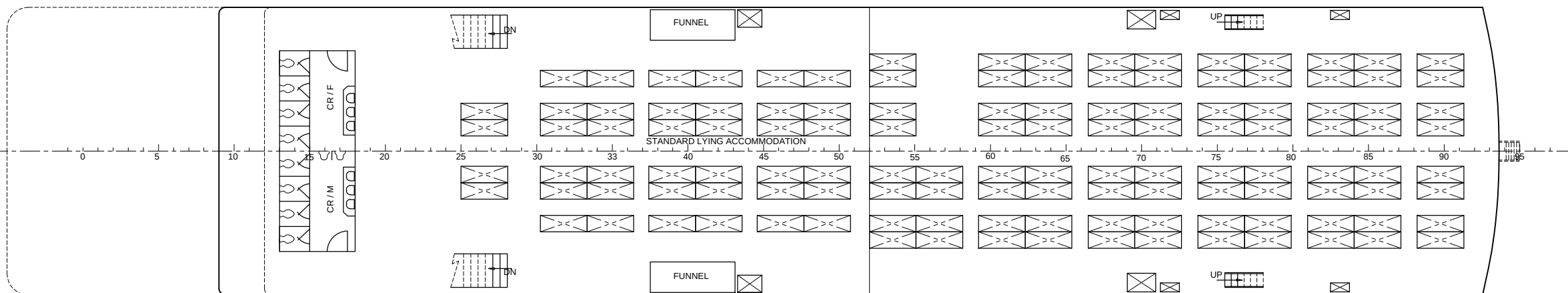
DECK - A PLAN
