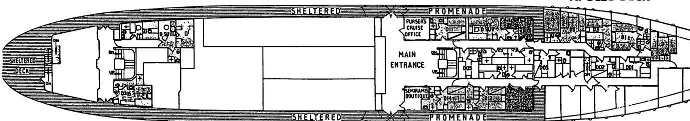
DIONYSOS DECK
