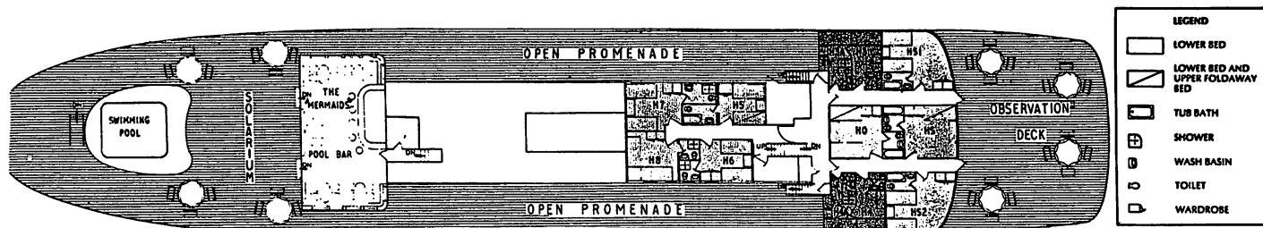
HERA DECK
