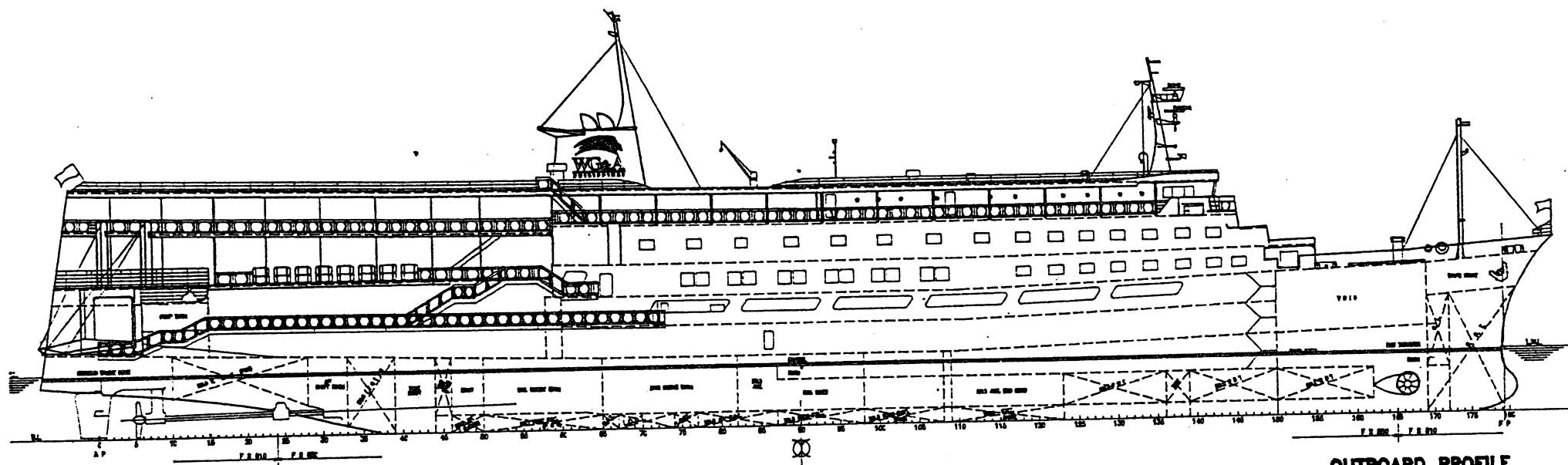
OUTBOARD PROFILE
