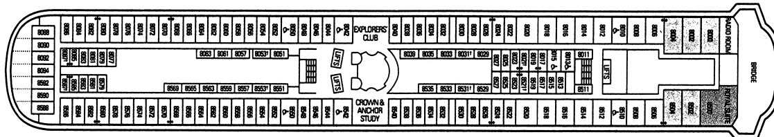
BRIDGE DECK
