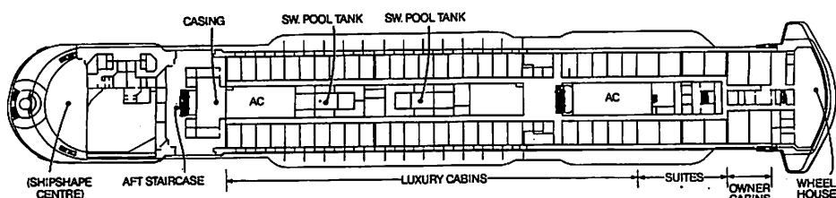
DECK 10
