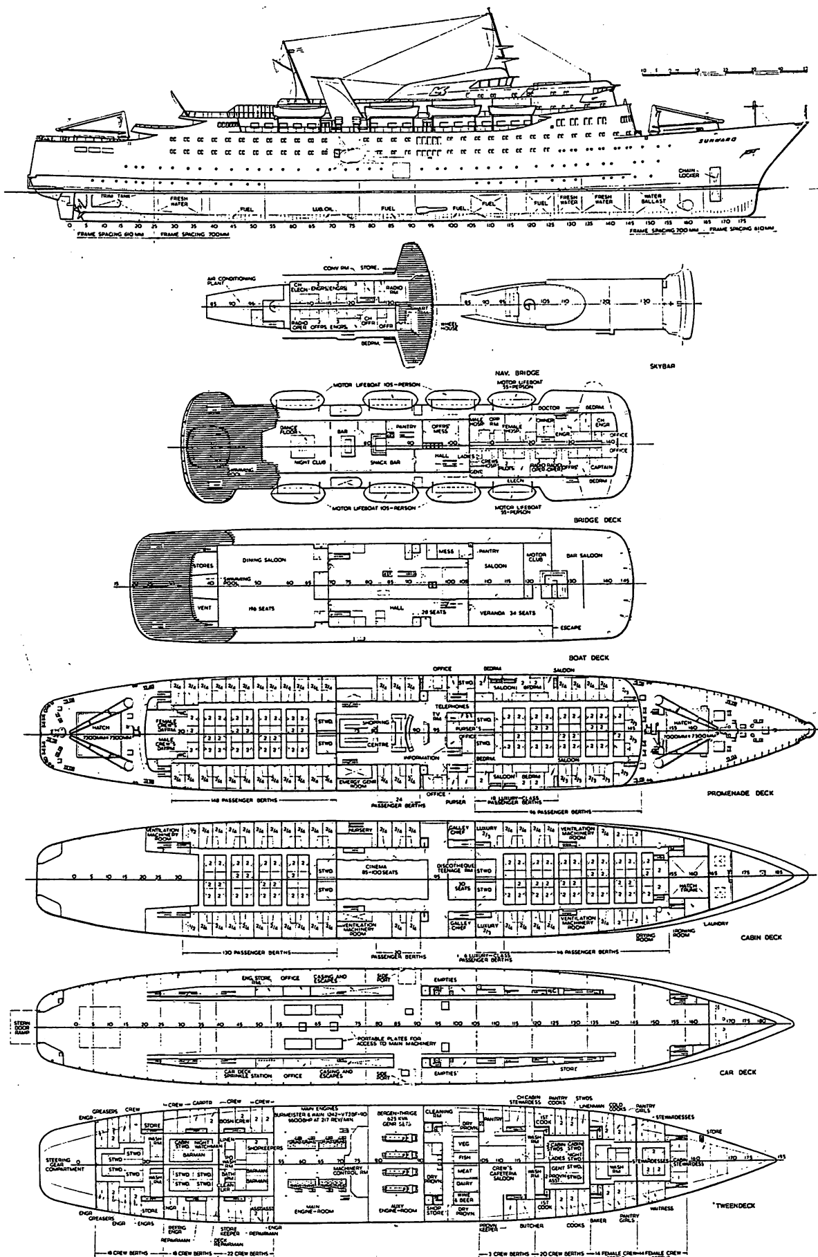
GENERAL ARRANGEMENT DRAWINGS OF THE KLOSTERS FERRY 'SUNWARD'
