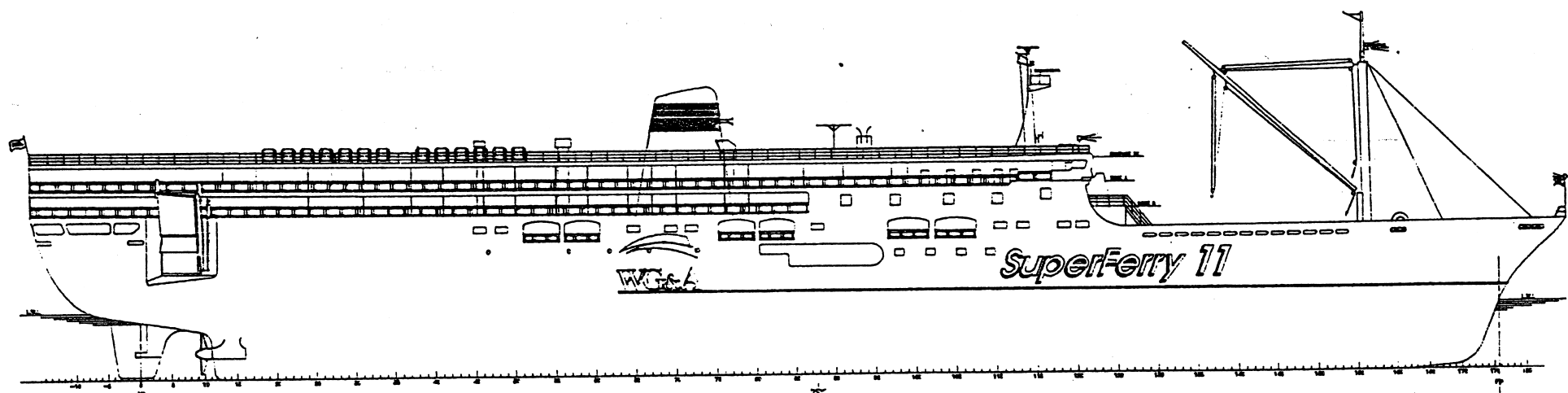
OUTBOARD PROFILE
