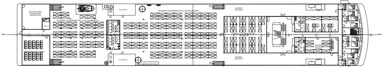
DECK A
