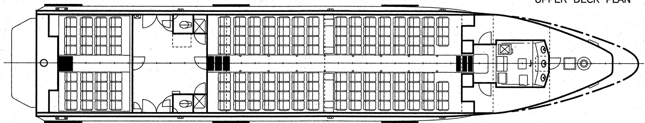
UPPER DECK PLAN
